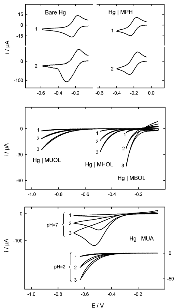
Figure 2. Cathodic stripping voltammograms recorded in solutions containing 100 \mu\text{M} corresponding thiol, 0.25 \text{ M H}_3\text{PO}_4 , pH 7, except for pH 2 solutions in the lowest panel, and (1) 1 \text{ mM Ru}(\text{NH}_3)_6^{3+} , (2) 5 \text{ mM Ru}(\text{NH}_3)_6^{3+} and (3) 10 \text{ mM Ru}(\text{NH}_3)_6^{3+} at the HMDE. Scan rate \nu = 1 \text{ V s}^{-1} , deposition potential E_d = -0.05 \text{ V} , and deposition time 100 \text{ s} . The nature of the thiol monolayer, if present, is indicated on each panel.
